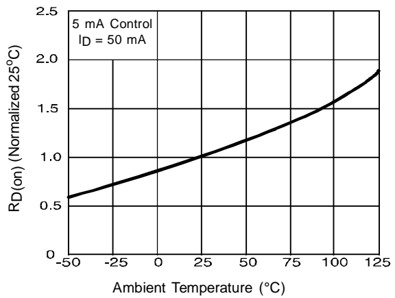
Figure 4. Typical On-Resistance
